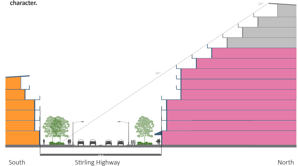
Figure 36: Stirling Highway (variable width) is characterised as a key primary regional road connection with moderate opportunity for treed edges to enhance amenity of separated pedestrian movement framed with 4 storey podium building edges and no street setbacks. Development form on the north shall limit overshadowing of the pedestrian environment on the southern verge.
