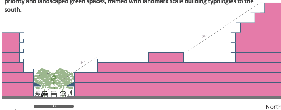
South St Quentin Avenue North Figure 27: Section B - St Quentin Avenue (12.0m) characterised as a slow speed pedestrian space framed by human scale buildings and no street setbacks.
