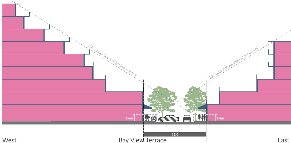
West Bay View Terrace East Figure 28: Section C - Bay View Terrace - north (15.0m) characterised by single storey heritage facade (east) with nil podium setbacks and upper level street setbacks determined by specified sight lines.
