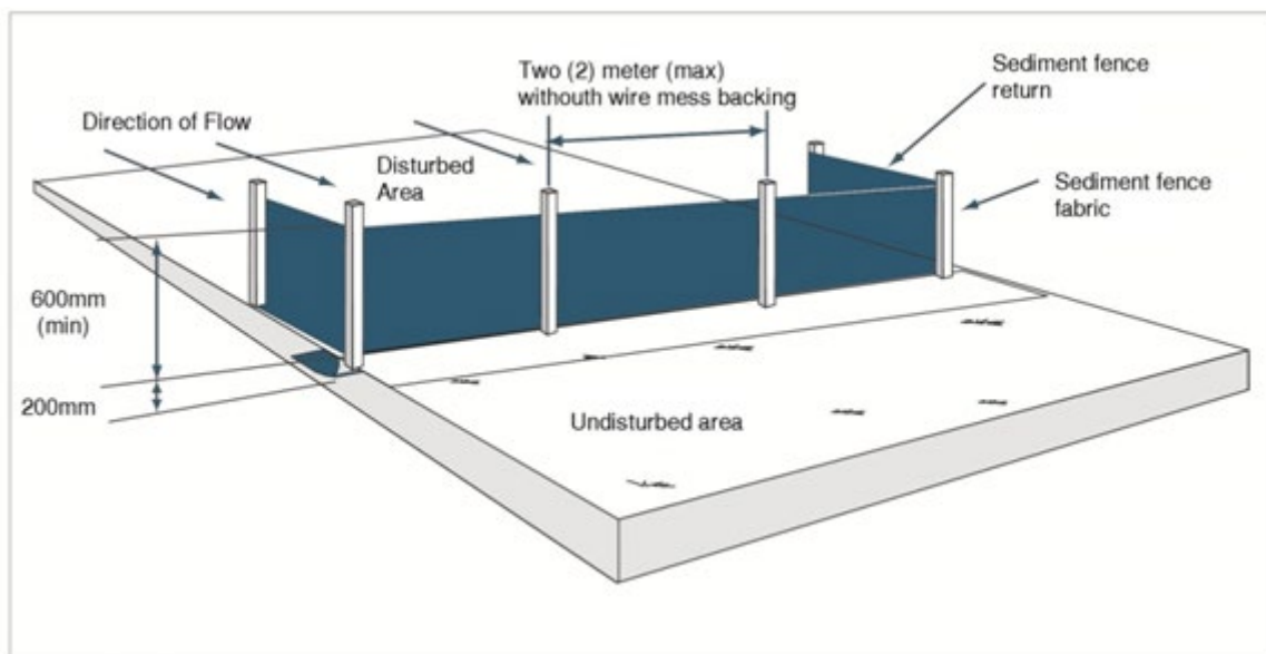
Figure 4: Typical sediment fence installation
